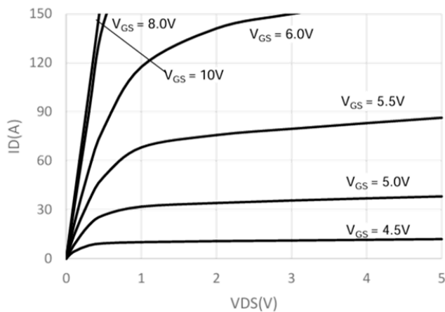
Output Characteristics
