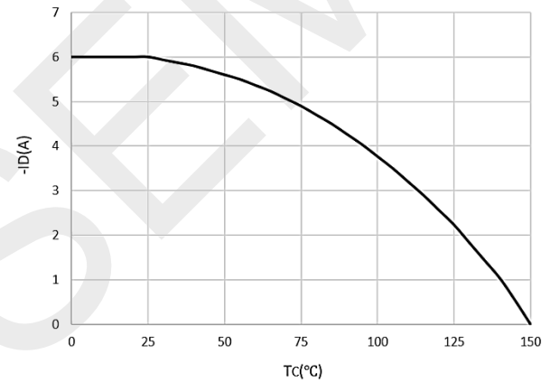
Current De-rating
