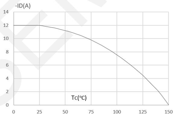
Current De-rating
