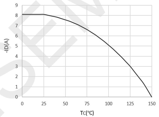
Current De-rating
