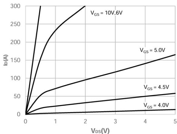
Saturation Characteristics
