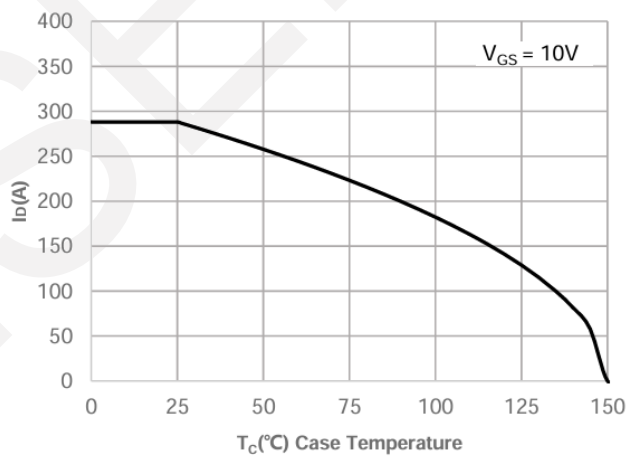
Current De-rating
