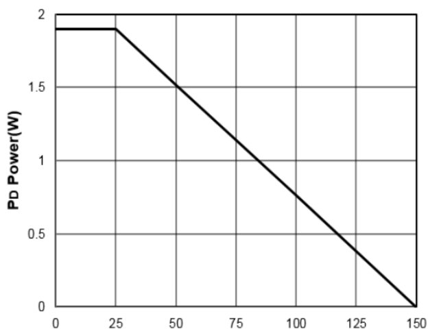
Power De-rating
