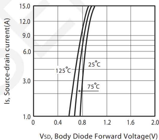
Body Diode Characteristics
