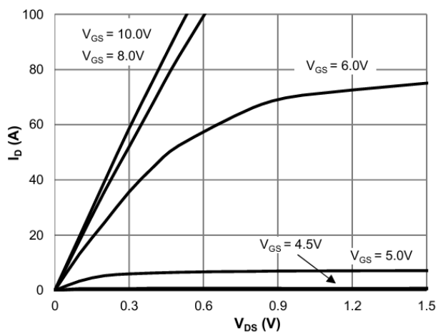
Saturation Characteristics
