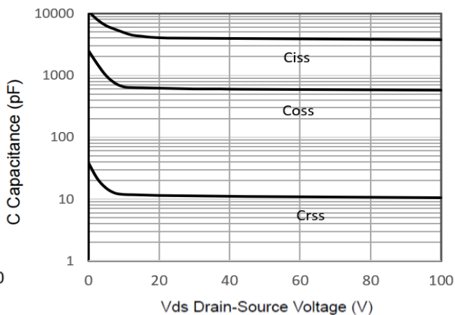
Capacitance Characteristics
