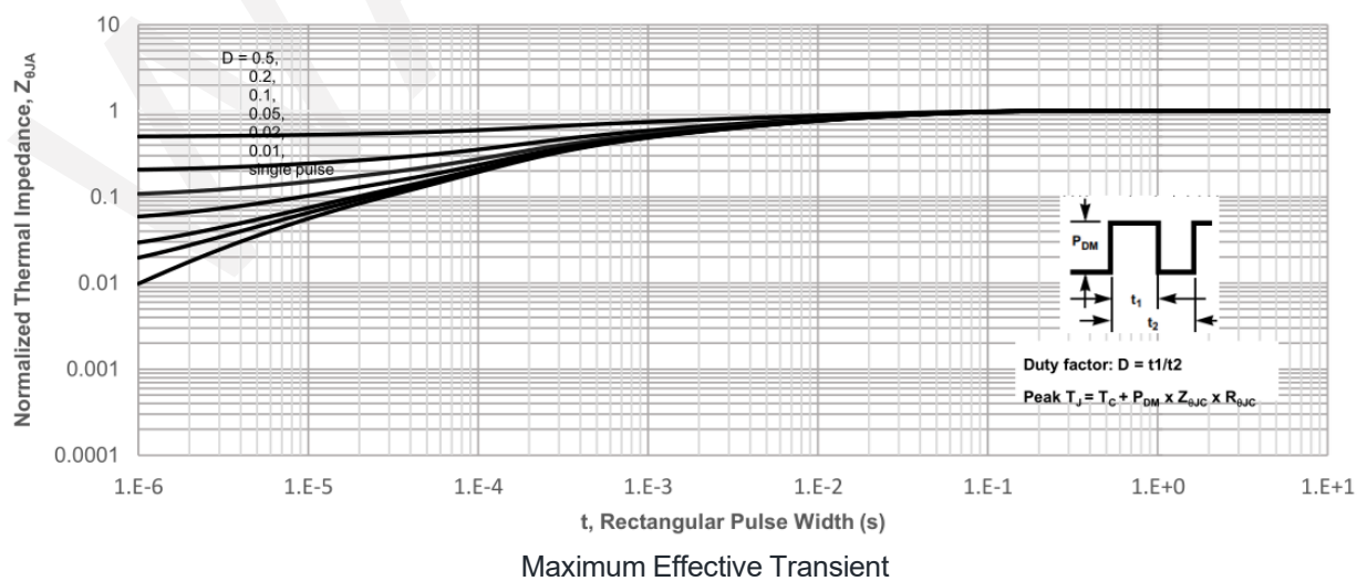
Thermal Impedance, Junction-to-Case
