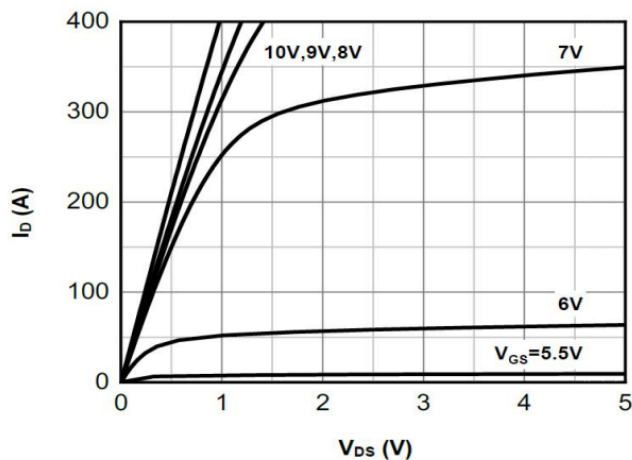
Saturation Characteristics
