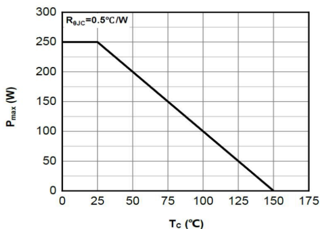
Power De-rating
