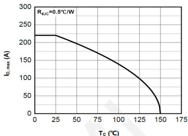
Current De-rating
