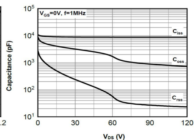
Capacitance Characteristics
