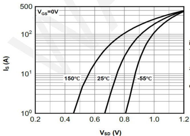
Body-Diode Characteristics
