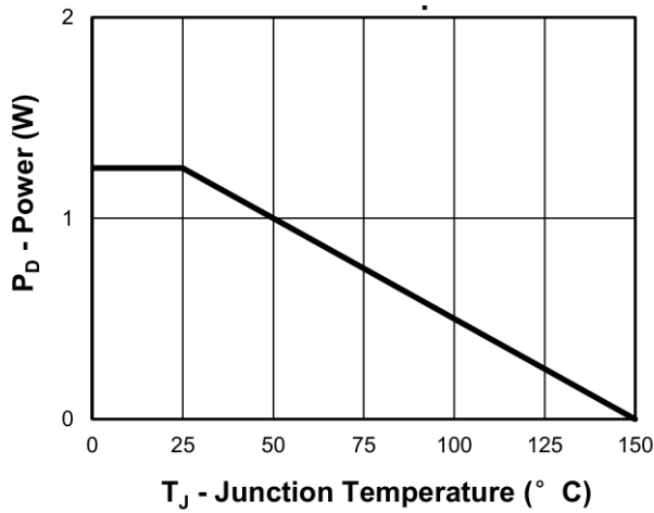
Power Dissipation
