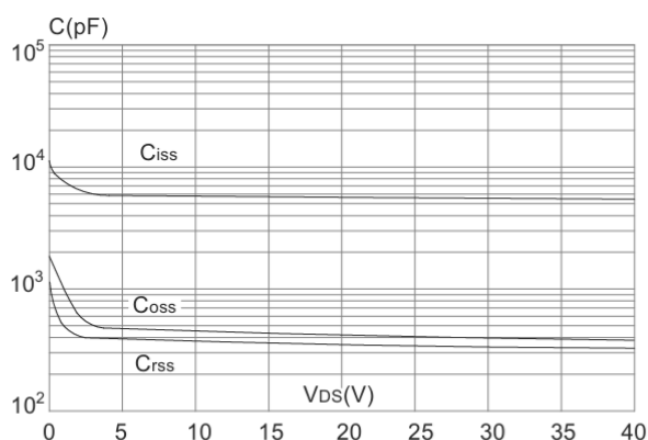
Capacitance Characteristics
