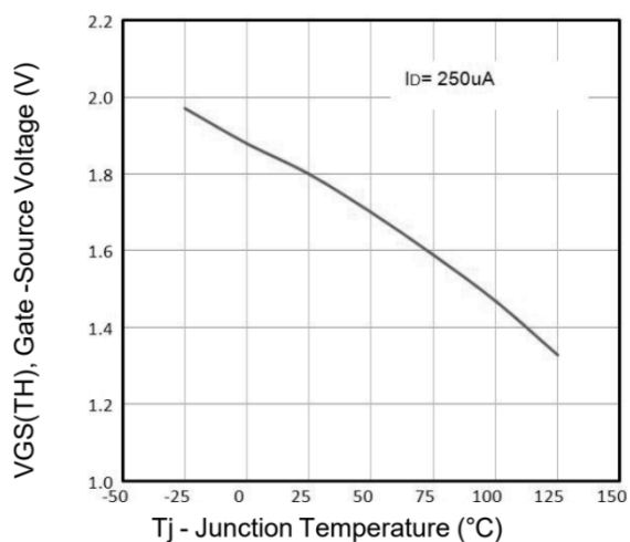
VGS(TH) Voltage Vs. Temperature
