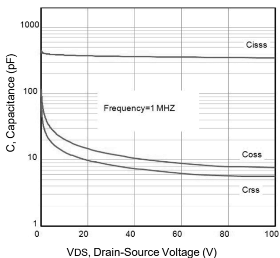
Capacitance Characteristics
