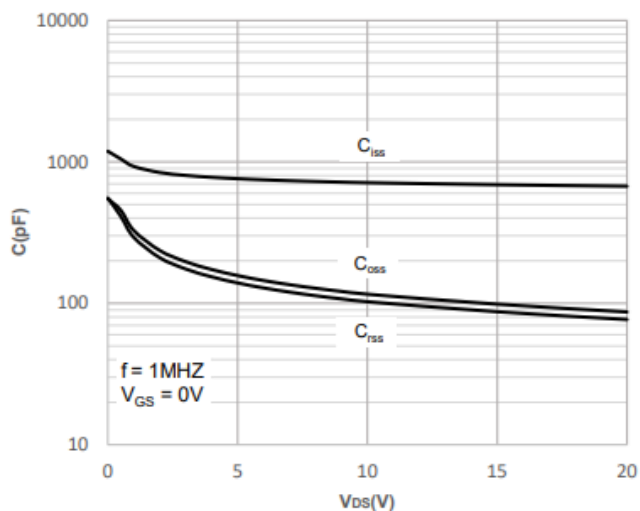
Capacitance Characteristics
