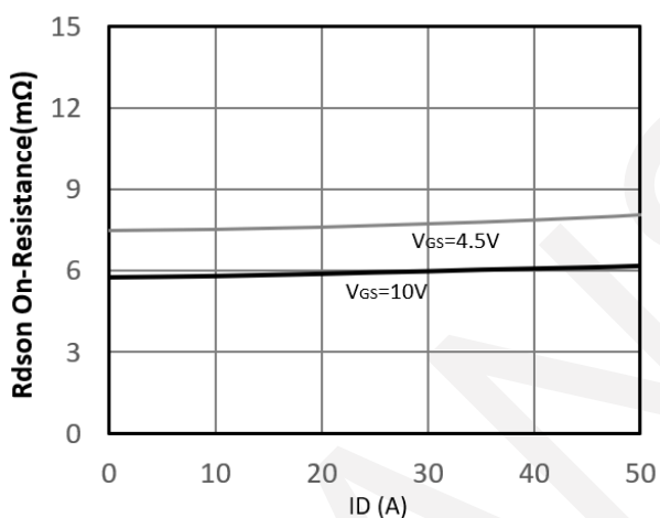
Rdson-Drain Current
