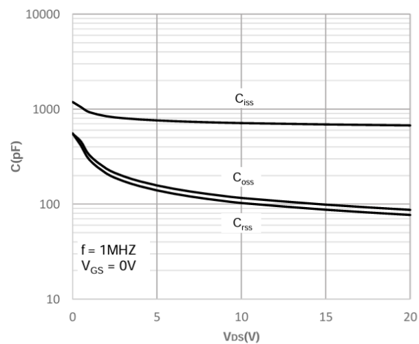
Capacitance Characteristics
