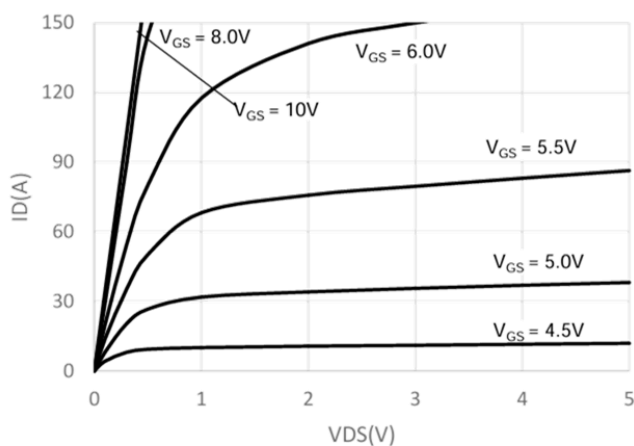
Saturation Characteristics
