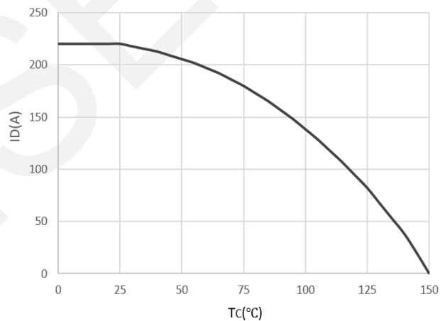
Current De-rating
