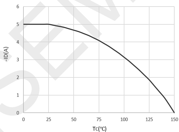
Current De-rating
