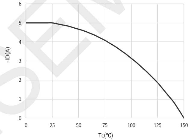
Current De-rating
