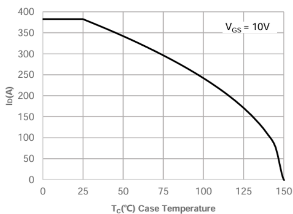
Current De-rating
