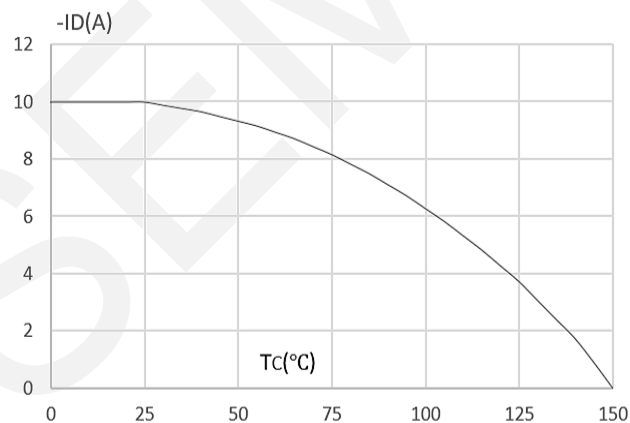
Current De-rating
