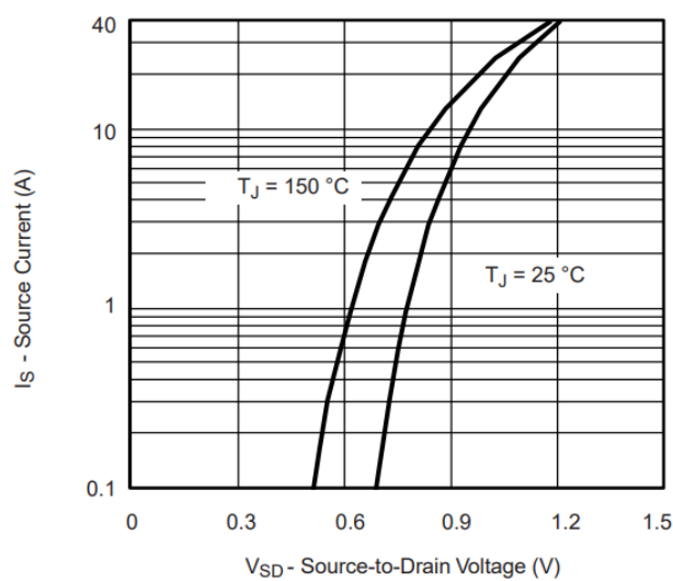
Figure 6 Body-Diode Characteristics
