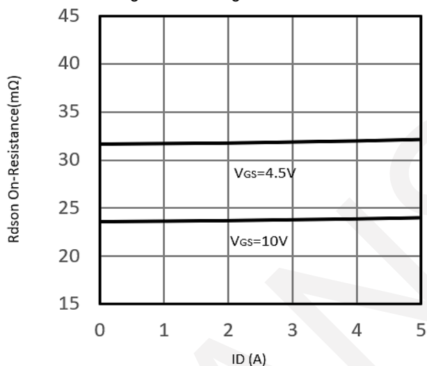
Figure 3 On-Resistance vs. Drain
