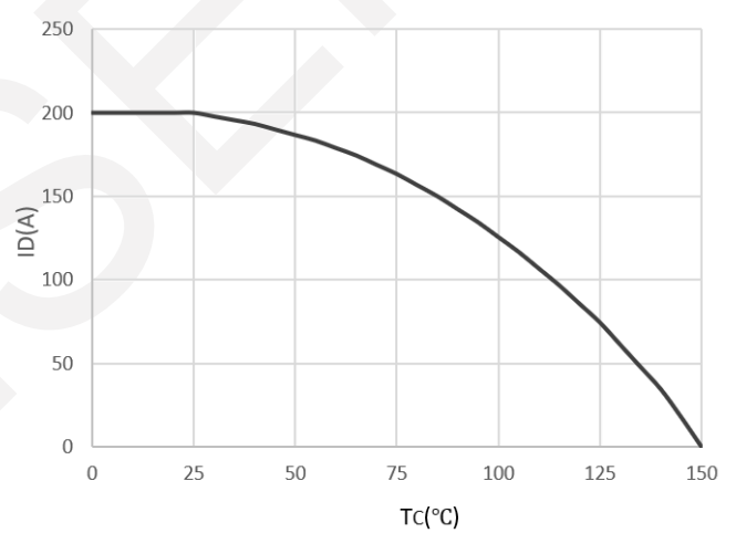
Current De-rating
