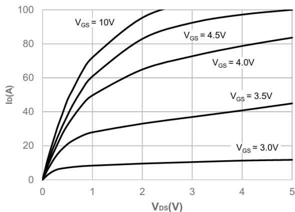
Output Characteristics
