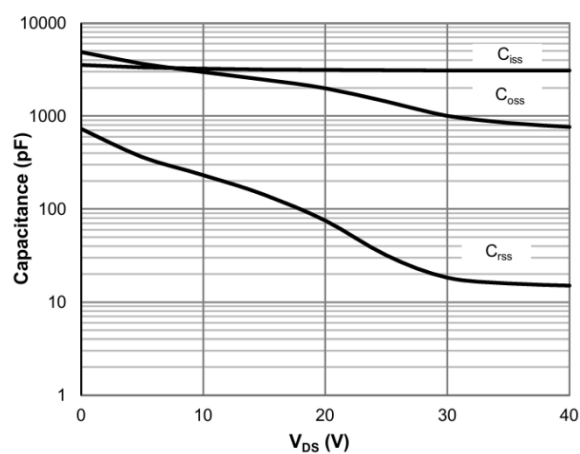
Capacitance Characteristics
