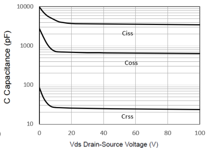
Capacitance Characteristics
