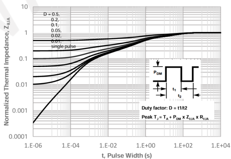
Figure 11 Normalized Maximum Transient Thermal Impedance WAN SEMICONDUCTOR (NINGBO) CO.,LTD
