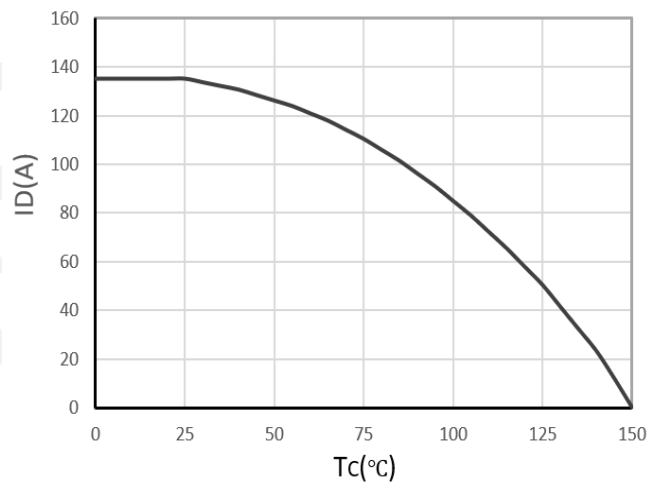
Current De-rating
