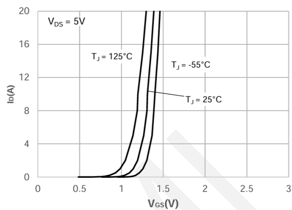
Transfer Characteristics
