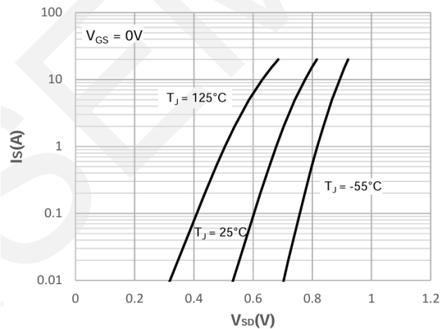
Body Diode Characteristic
