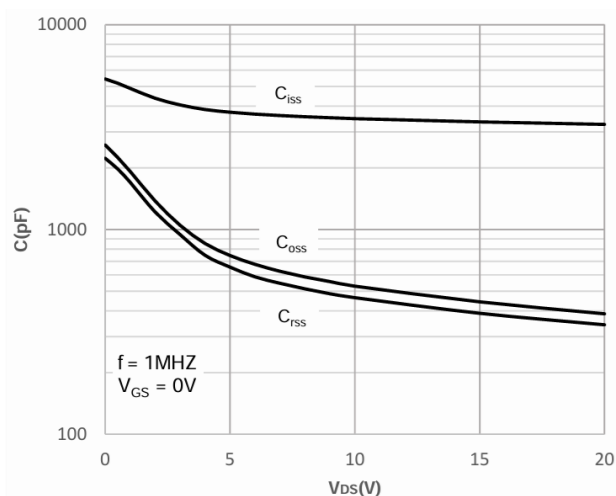
Capacitance Characteristics
