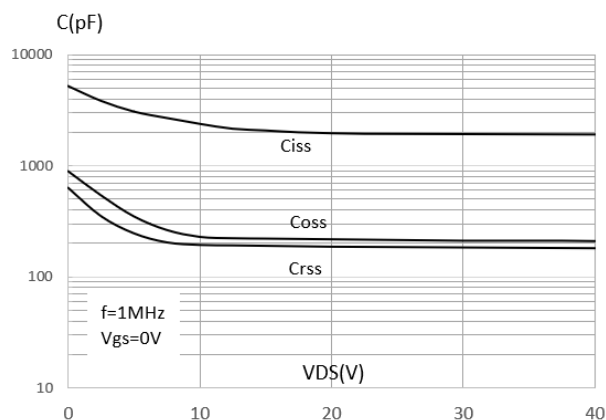
Capacitance Characteristics
