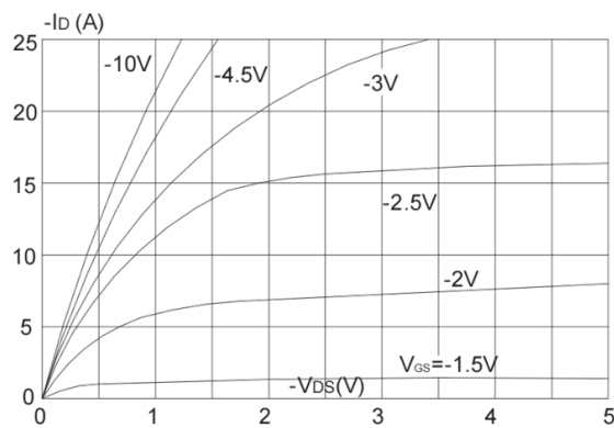
Output Characteristics
