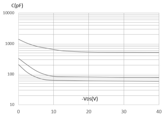
Capacitance Characteristics
