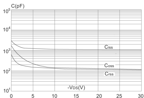
Capacitance Characteristics
