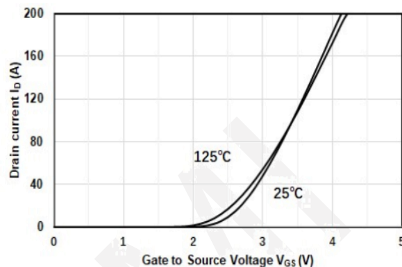
Transfer Characteristics
