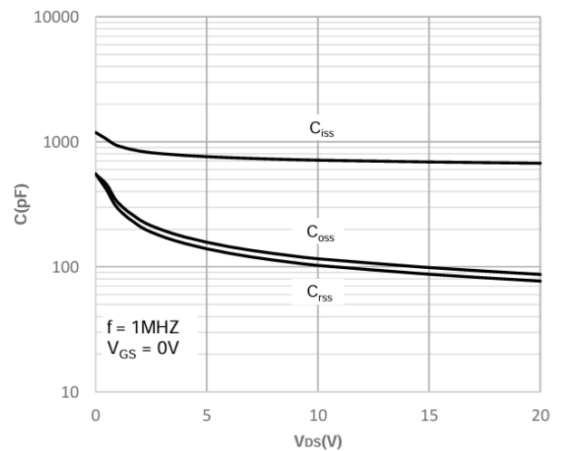
Capacitance Characteristics
