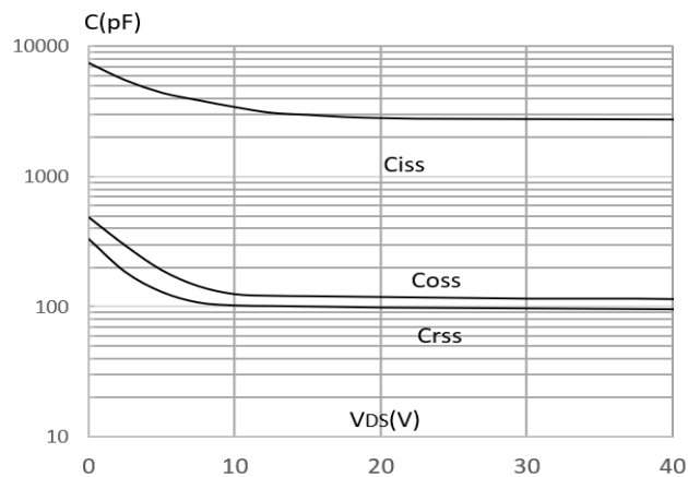
Capacitance Characteristics
