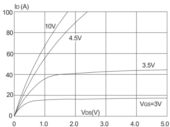
Output Characteristics
